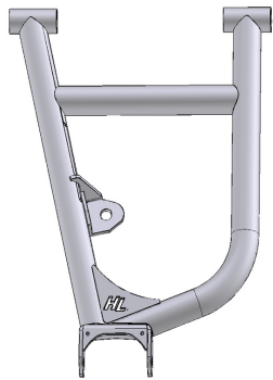
130T-L Rear Upper Left Control Arm (1ea)
