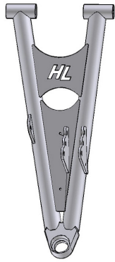
129A-L Front Upper Left Control Arm (1ea)
