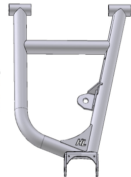
130T-R Rear Upper Right Control Arm (1ea)
