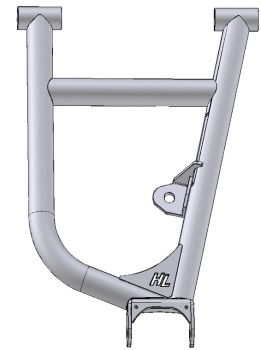
130T-R Rear Upper Right Control Arm (1ea)
