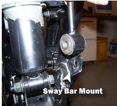
LOWER SWAY BAR LINK END
