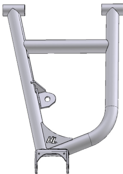
130T-L Rear Upper Left Control Arm (1ea)
